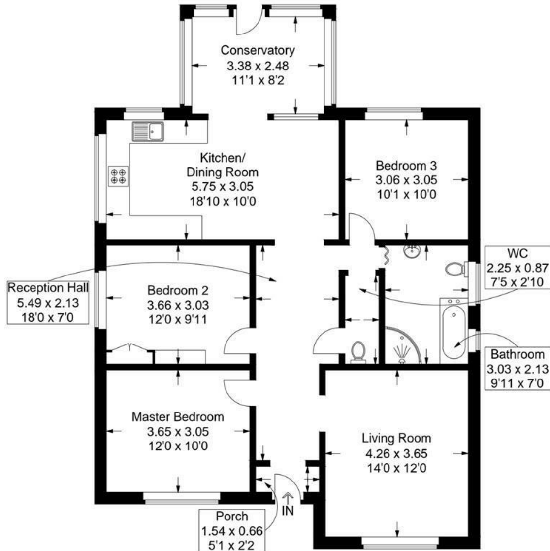
Ground Floor
